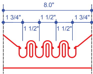
8" Corner 45° Block Outside Corner Side Elevation
