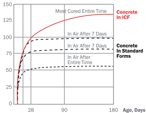
Graph showing hydration at work. (Courtesy of Portland Cement Association)
